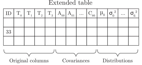
Fig. 5. The result of CPA. Every lookup for a row yields a value, such as \mu_5 or B_{43} . The values form their own columns, resulting in an extended table.
