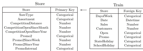
Fig. 10. The schema from the Rossmann Store dataset. Each store is a different store location of the Rossmann franchise, and each row in Train corresponds to a particular day in the store.
